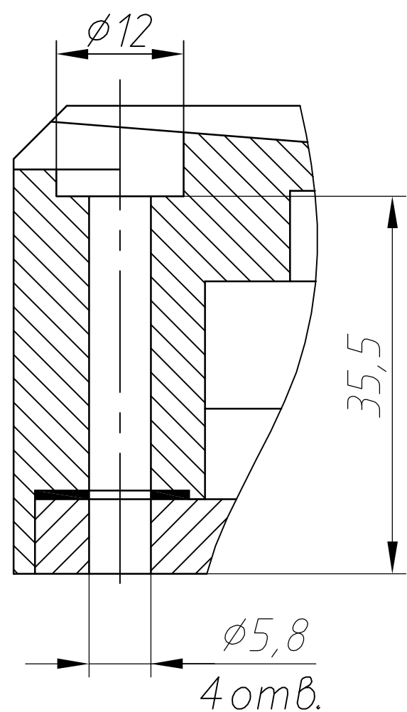
В—В(1:1)
